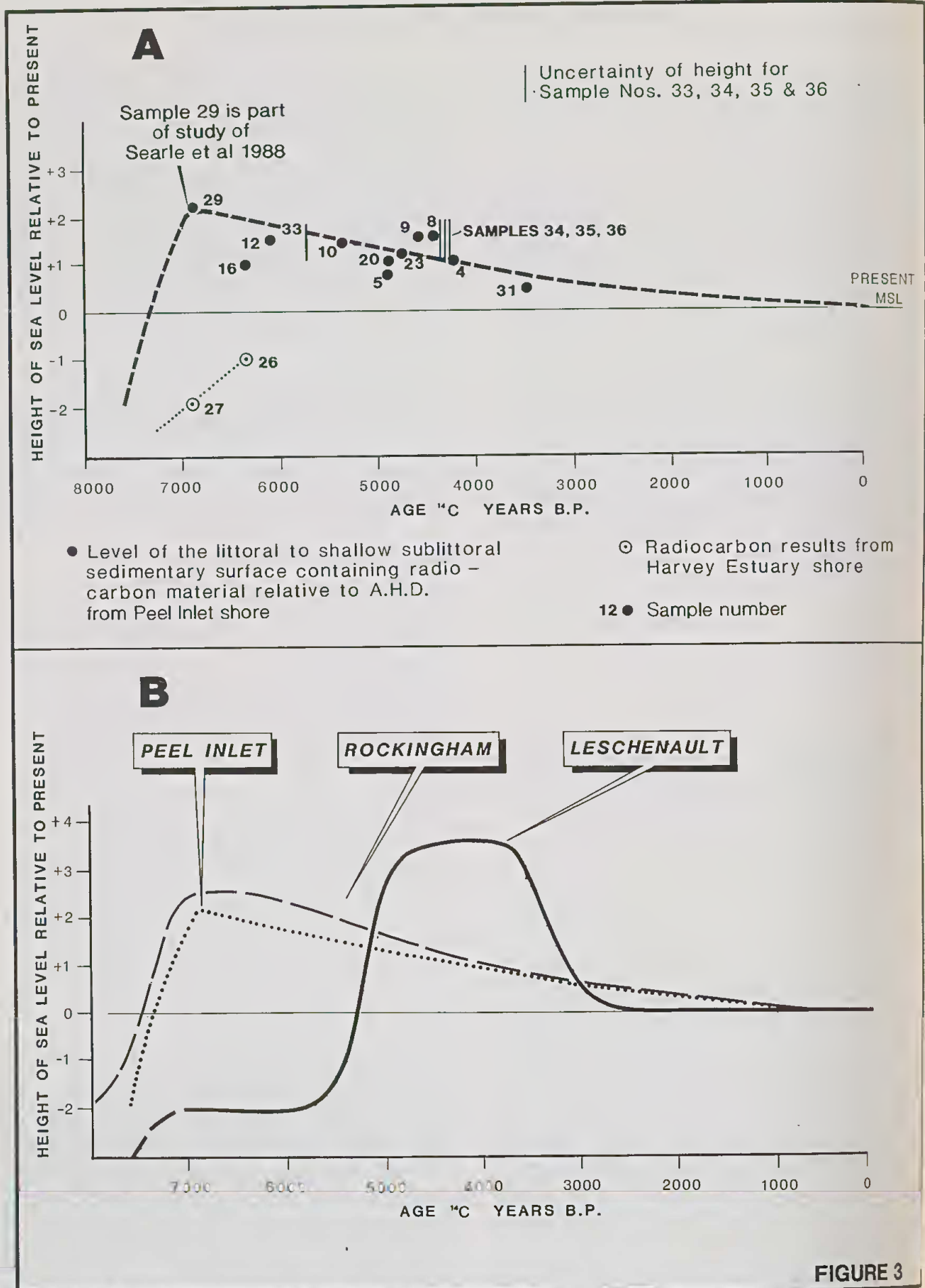
Figure 3 A Sealevel history curve for the Peel-Harvey estuary. B Sealevel history curve for the Peel-Harvey estuary compared to sealevel history of the Leschenault Peninsula and Rockingham-Becher areas (after Semeniuk & Searle 1986). Note that the curve from Searle et al. 1988 has had the reservoir correction factor removed to make it comparable with the curves of this study and with Semeniuk 1985. The radiocarbon results of Semeniuk 1985 had not been corrected by Semeniuk for oceanic reservoir effects because that study too was based mainly on estuarine shell.
